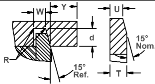
Exploded Groove Profile & Edge Margin (Y) Maximum bottom radii (R), .005 for ring sizes -100 thru -200; .010 for ring sizes -206 thru -1000
