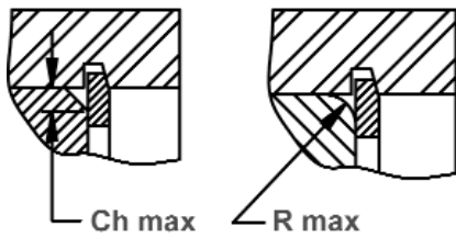
Allowable Corner Radius & Chamfer
