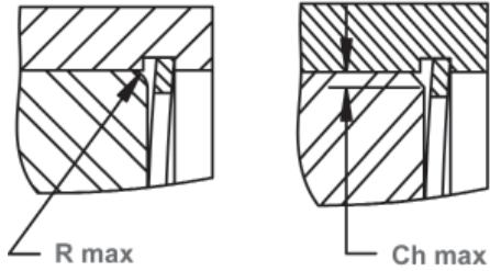
Maximum Corner Radius & Chamfer
