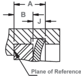
Outer Groove Location A max = B min + J max A min = B max + J min
